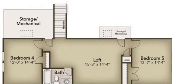
Finished Second Floor (with or without bedroom 5)
